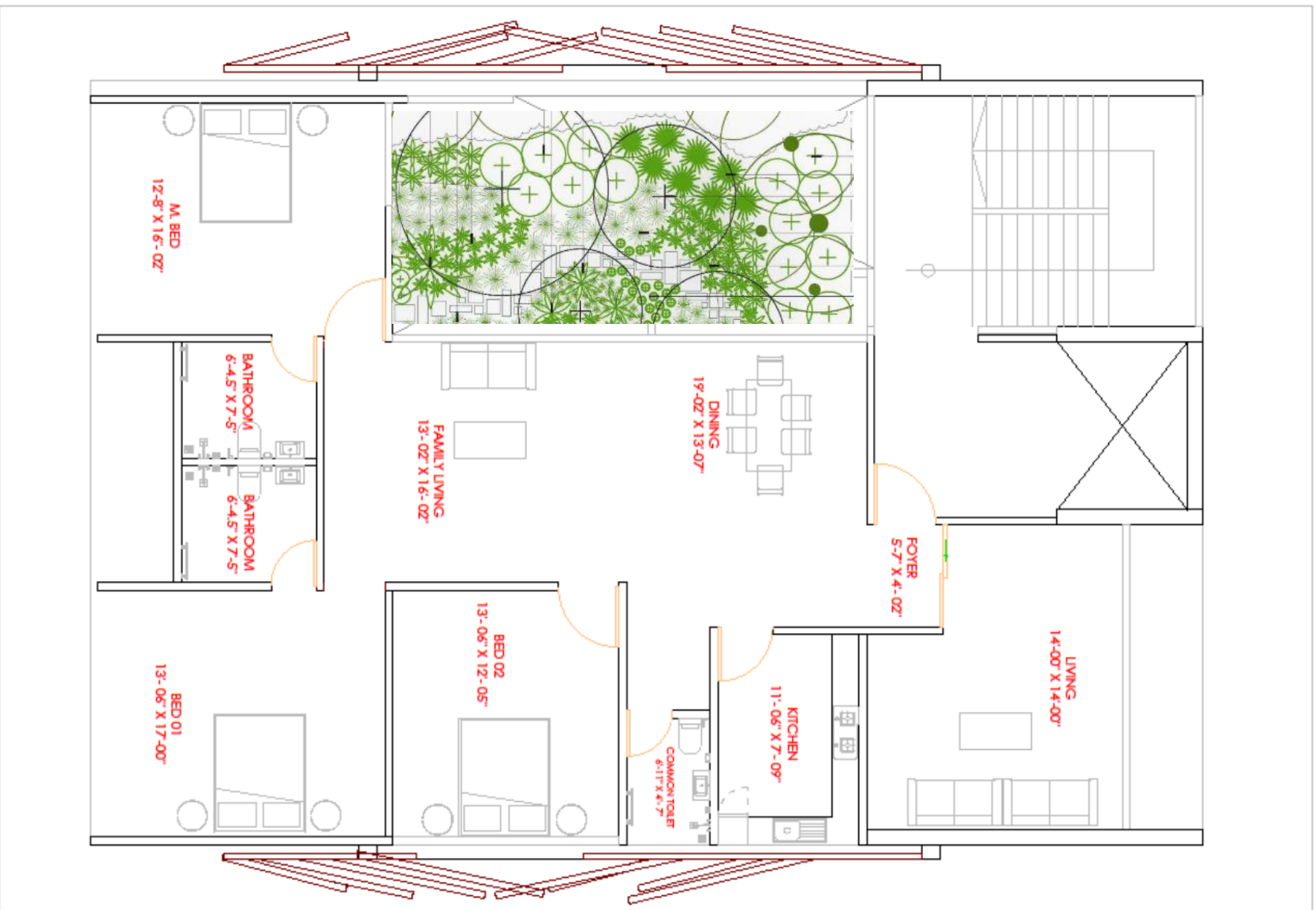
Typical Floor
